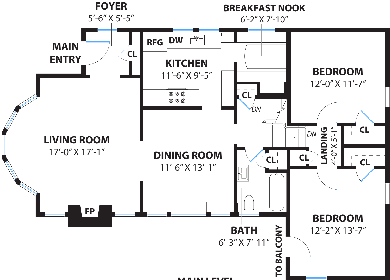
MAIN LEVEL
